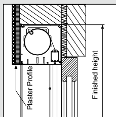
Hidden Installation with box Stucco
