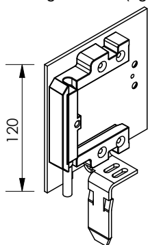
Mounting feet 120 (right)
