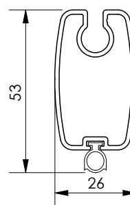
Bottom rail
