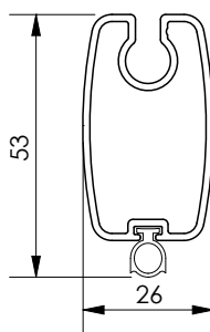
Bottom rail
