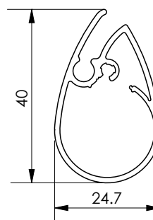
Bottom rail
