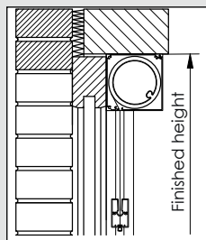
Surface-mounted Inside, in front of the window
