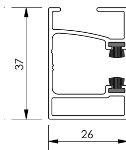
Side channel for reversed box mounting O
