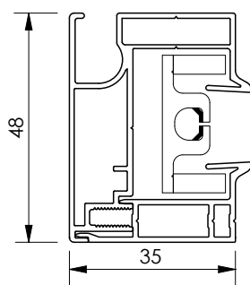
Open side channel Fixscreen® S
