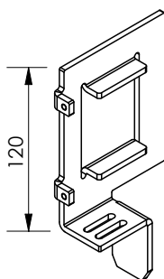
Mounting feet 120 (right side)
