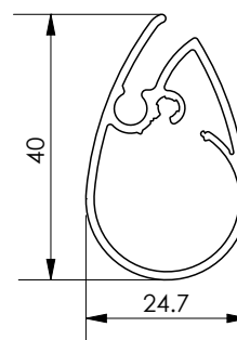
Bottom rail
