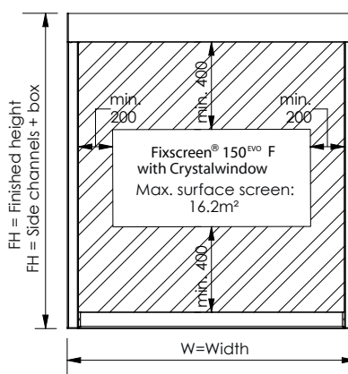
Deep side channel D
