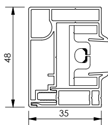
Closed Side channel G
