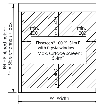
Surface mounted with box
