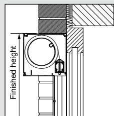
Surface mounted with box (closed side channel)
