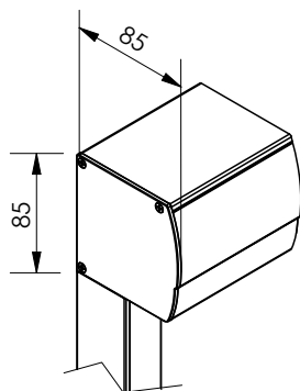
Side channel Fixscreen® S
