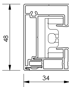
Side channel Fixscreen® S
