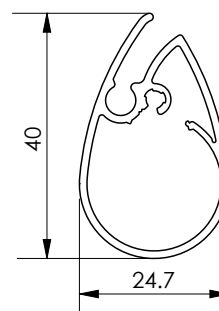
Bottom rail
