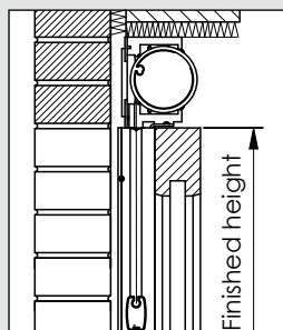
Hidden installation with brackets, without box
