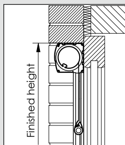
Surface-mounted Outside, in front of the window
