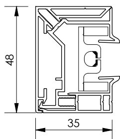
Closed side channel G
