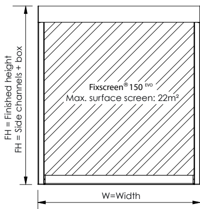
Surface mounted with box (deep side channel)
