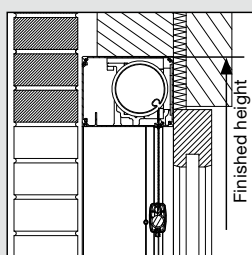
Hidden installation with box
