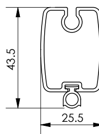
Bottom rail
