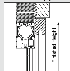
Surface mounted with box
