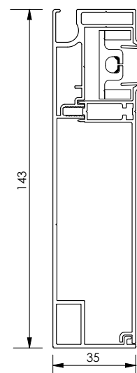
Diepe Side channel D
