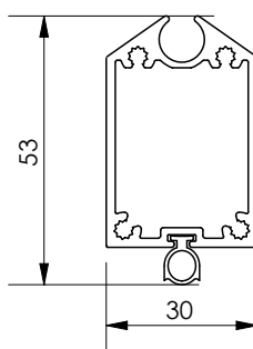
bottom rail
