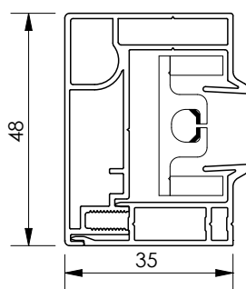
Closed side channel Fixscreen® G
