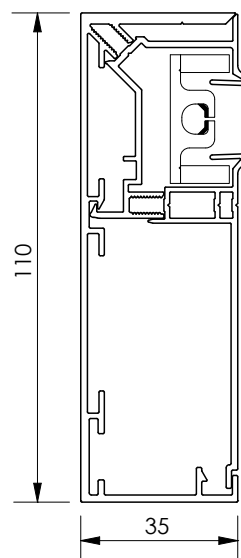
deep side channel D
