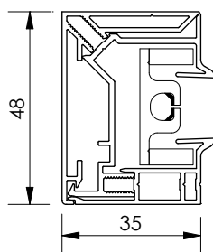
closed side channel G
