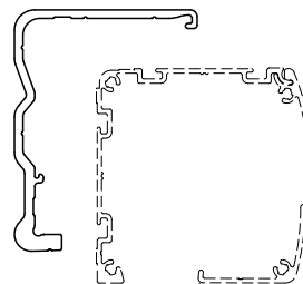
Clips
