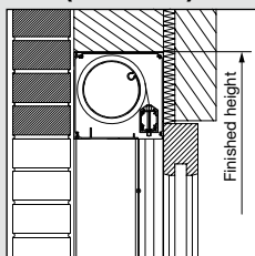
Surface mounted with box (deep side channel)
