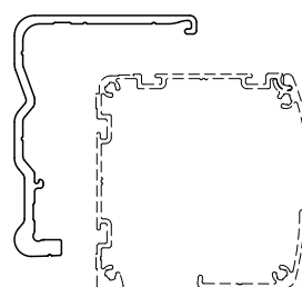
Clips
