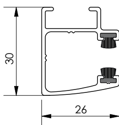
Side channel S
