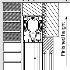
Hidden installation with box (Deep side channel)
