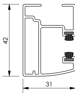
Side channel S
