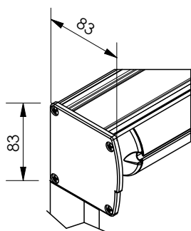
Side channel for reversed box mounting O
