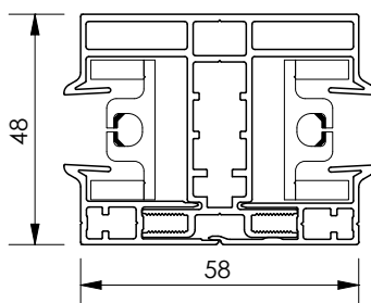
Coupled side channel K
