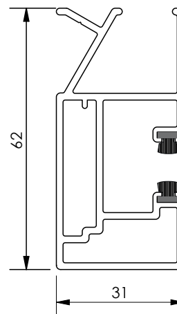
Side channel for reversed box mounting X
