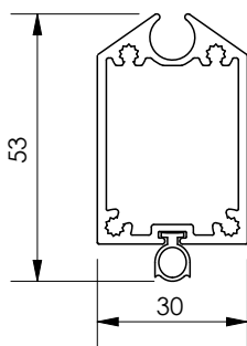
Bottom rail
