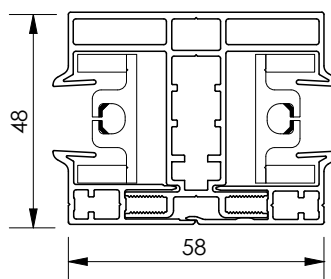
coupled side channel K
