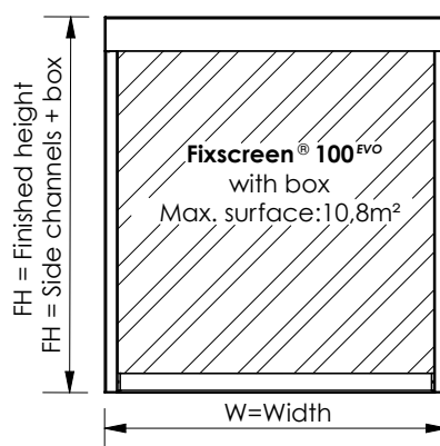
Hidden installation with box Stucco
