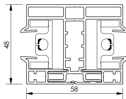
Coupled side channel Fixscreen® K
