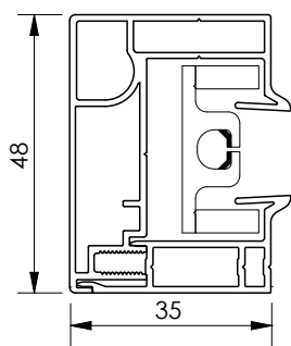
Side channel Fixscreen® S
