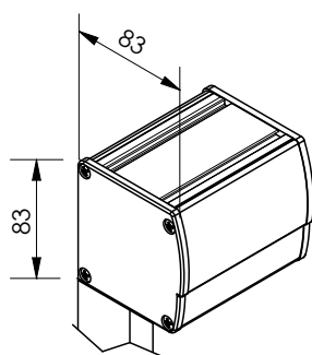
Side channel S
