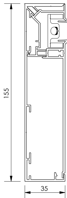
Deep side channel D
