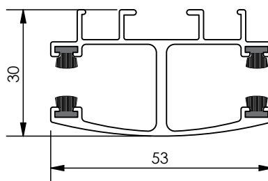
Coupled side channel K
