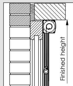
Surface mounted Inside, in front of the window
