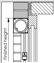
Surface-mounted Outside, in front of the window
