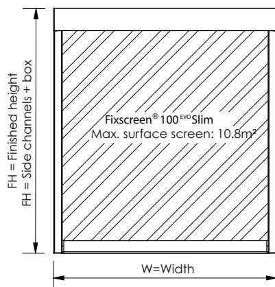
Hidden installation with box (Deep side channel)
