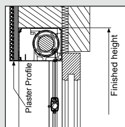
Hidden installation with box Stucco
