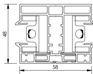
Coupled side channel K
