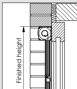
Surface mounted Outside, in front of the window
