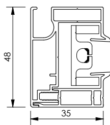
Open side channel S
