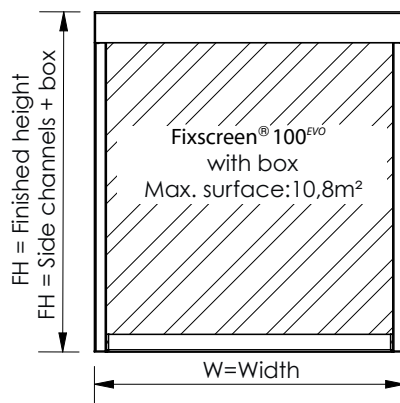
Surface-mounted Outside, in front of the window
