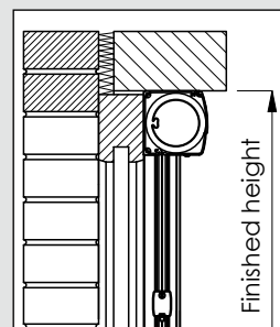
Surface-mounted Inside, in front of the window
