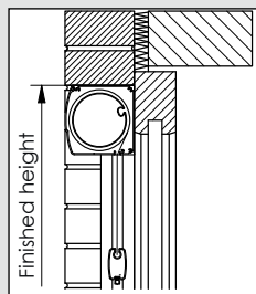
Surface-mounted Outside, in front of the window
